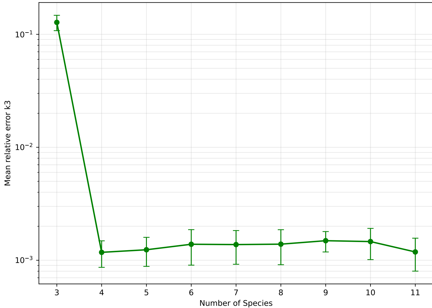
30, 30, 30 — Mean relative error k3 vs number of species (3 to 11 species)
